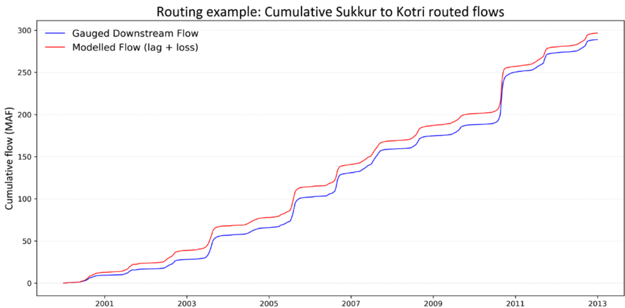
Figure 72 Kotri modelled and measured cumulative flow volumes
