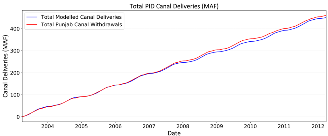
Figure 89 Cumulative modelled Punjab water entitlement and cumulative actual withdrawals
